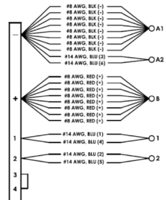
WIRE DIAGRAM
