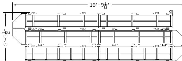
Typical 3-Section Configuration (603lbs)
