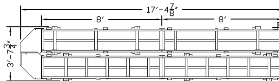
Typical 2-Section Configuration (395lbs)
